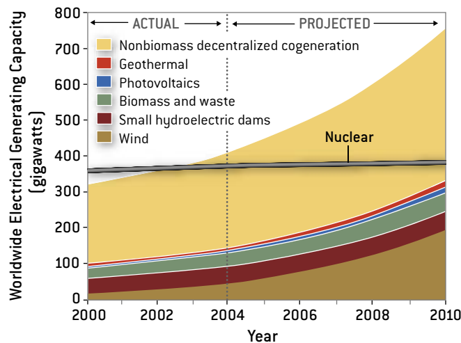
DECENTRALIZED SOURCES of electricity—cogeneration (the combined production of electricity and heat, typically from natural gas) and renewables (such as solar and wind power)—surpassed nuclear power in global generating capacity in 2002. The annual output of these low- and no-carbon sources will exceed that of nuclear power this year.
